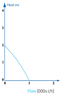
Reef Pump 1000
