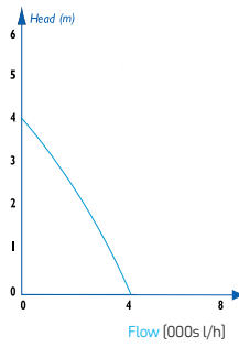
Reef Pump 4000
