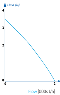
Reef Pump 2000
