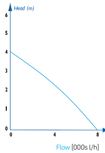
Reef Pump 8000
