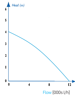
Reef Pump 12000
